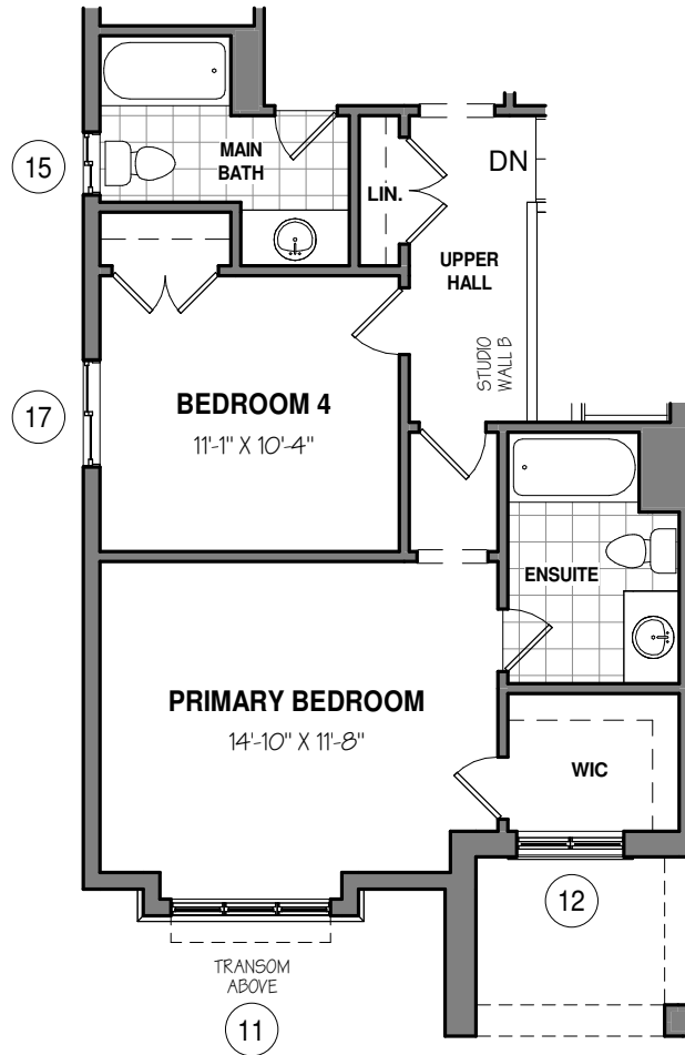
UPPER FLOOR
