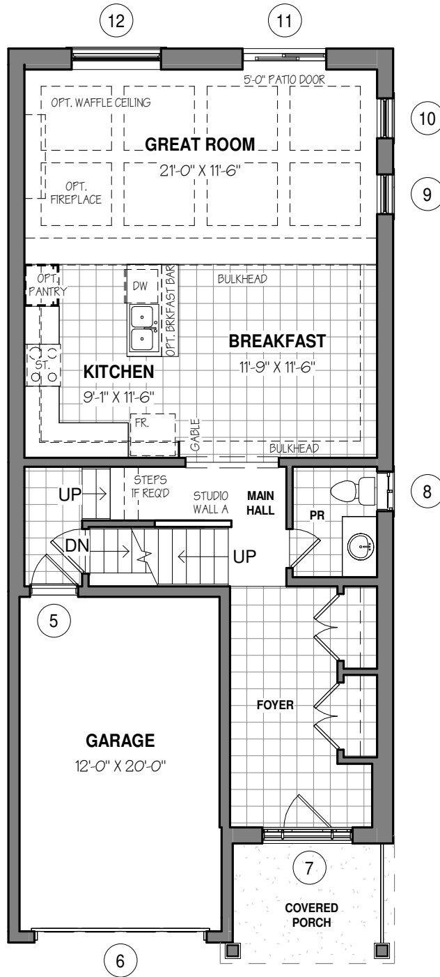
MAIN FLOOR PLAN MAIN FLOOR AREA 903 SF
