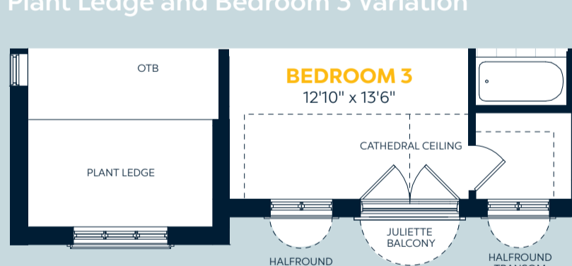
Elevation E Plant Ledge and Bedroom 3 Variation
