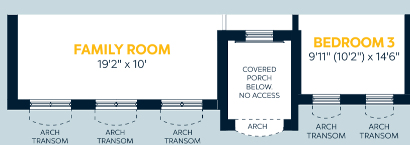
Elevation D Family Room and Bedroom 3 Variation
