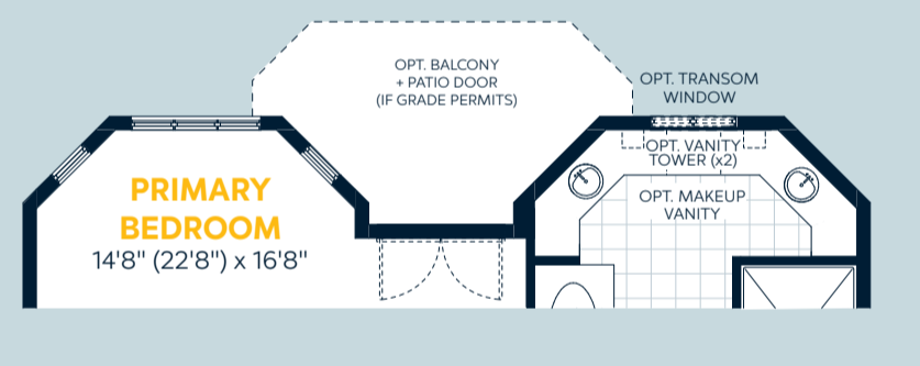
Primary Bedroom & Ensuite Variation
