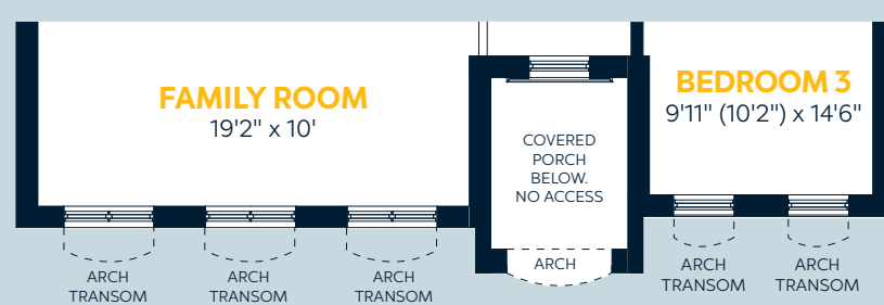
Elevation D Family Room and Bedroom 3 Variation
