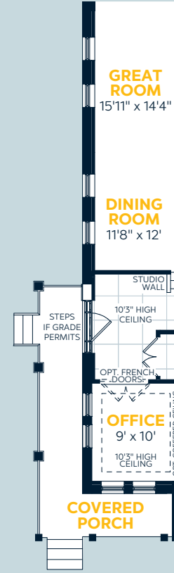
Main Floor Variation
