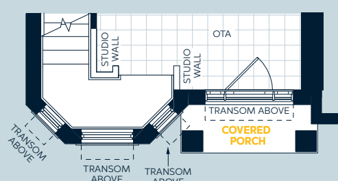
Elevation C Porch and Stair Landing Variation
